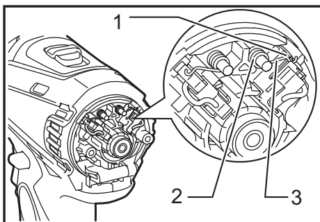
► 1. Recessed part 2. Spring 3. Arm
